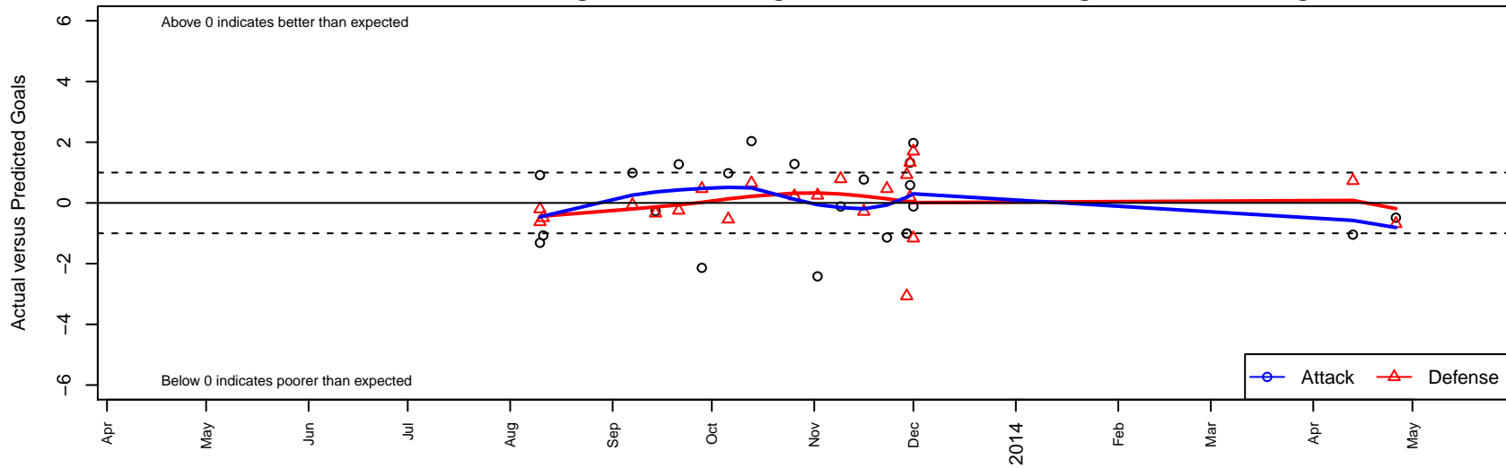
Downtown SC B98 Dots are actual minus expected GF (blue circles) and GA (red triangles). Blue line is smoothed change in attack strength. Red is smoothed change in defense strength.
